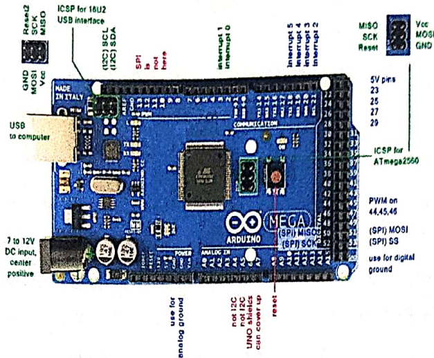
Fig 3.2: ATmega2560 Microcontroller
